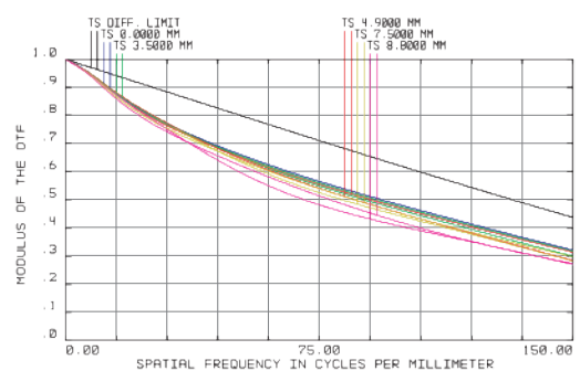
MTF
